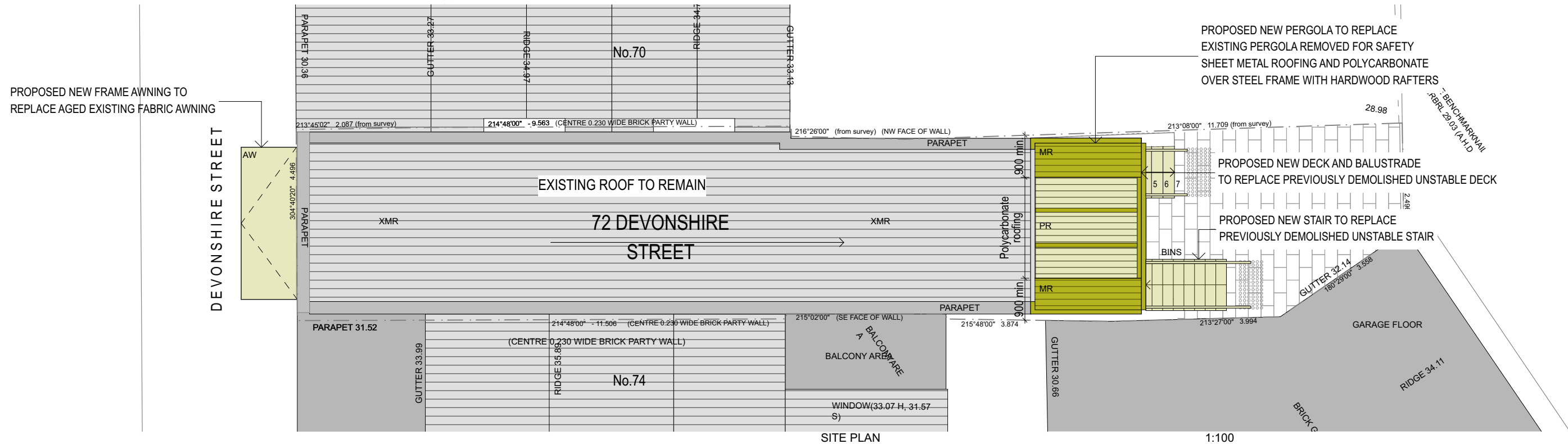
SITE PLAN
